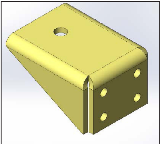
Pogo Wall Mount Bracket (ProCore Edge 9 / 15 / 30) P/N 5912678
