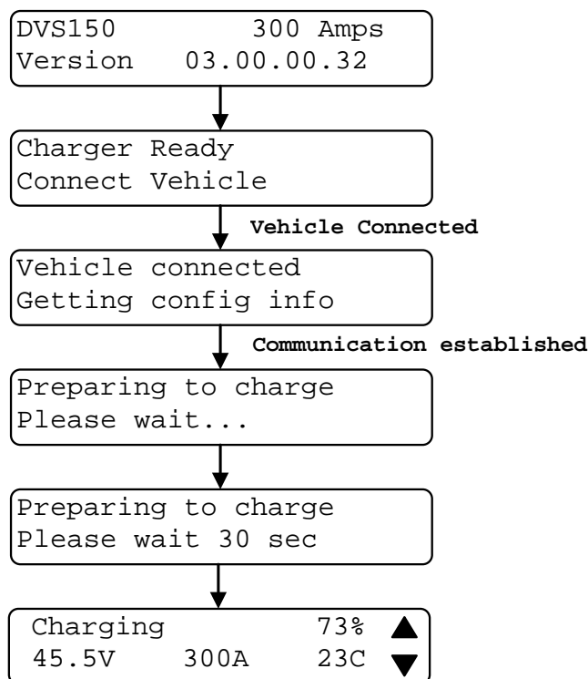
Figure 5- 3 Connecting Status Screens
