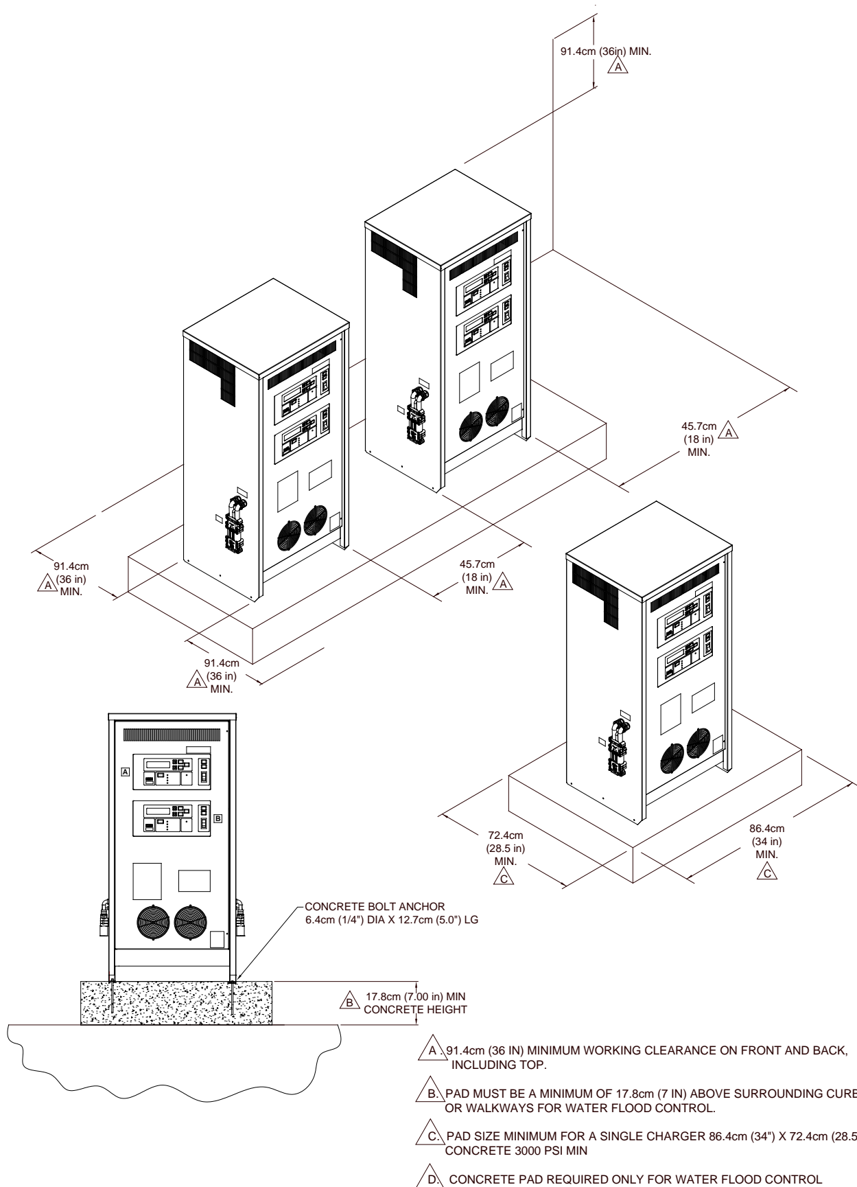
Figure 4- 1 DVS150 Installation
