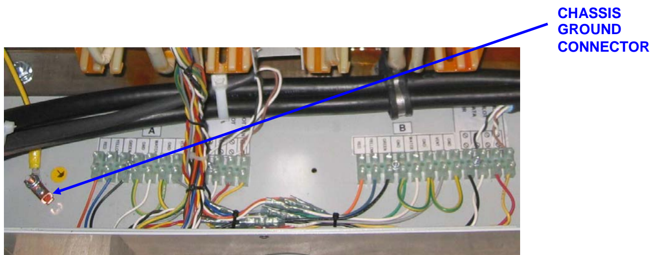
Figure 4- 3 AC Input Terminal Block
