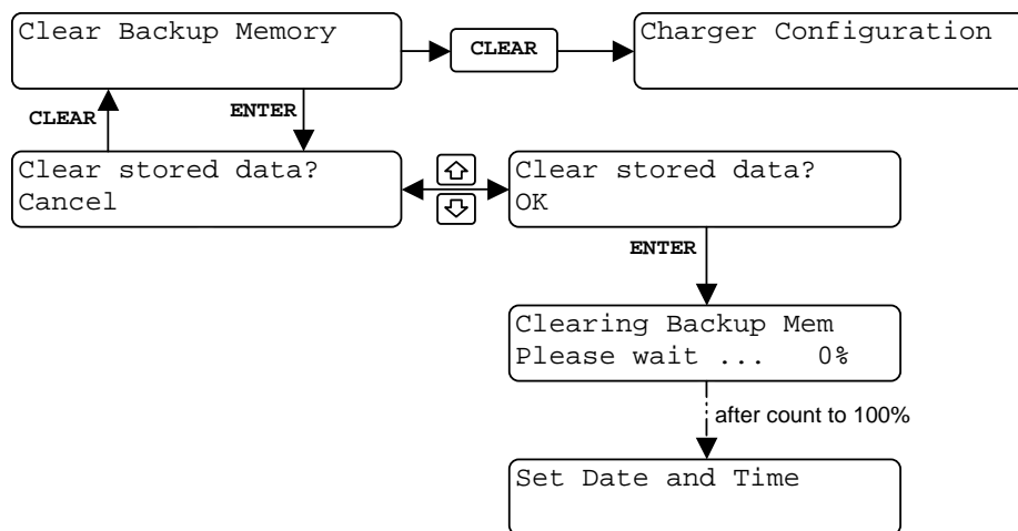
Figure 5- 13 Clear Backup Memory Menu
