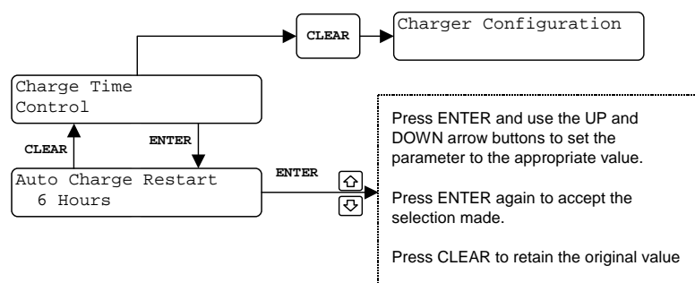
Figure 5- 26 Charger Time Control Menu
