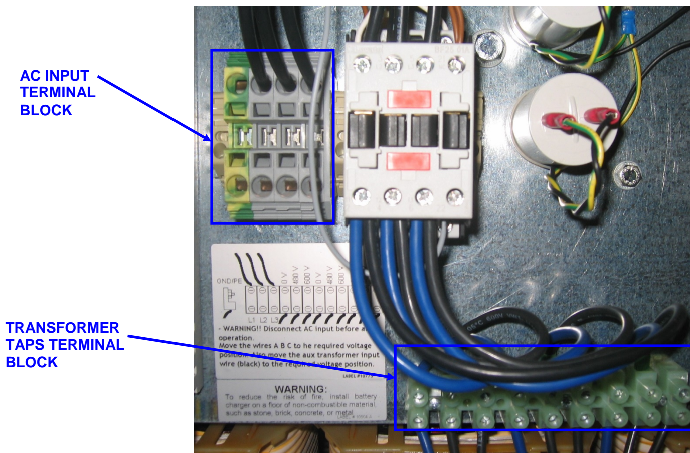
Figure 4- 3 AC Input Terminal Block
