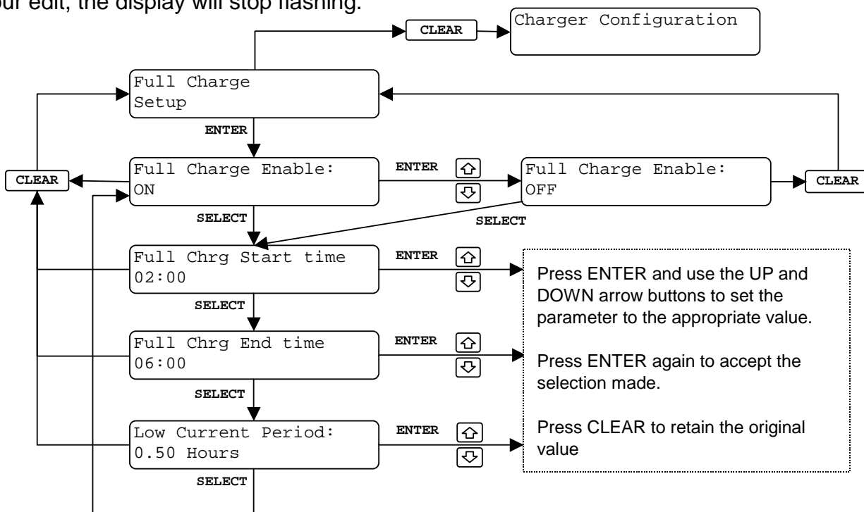
Figure 5- 18 Full Charge Setup Screens
