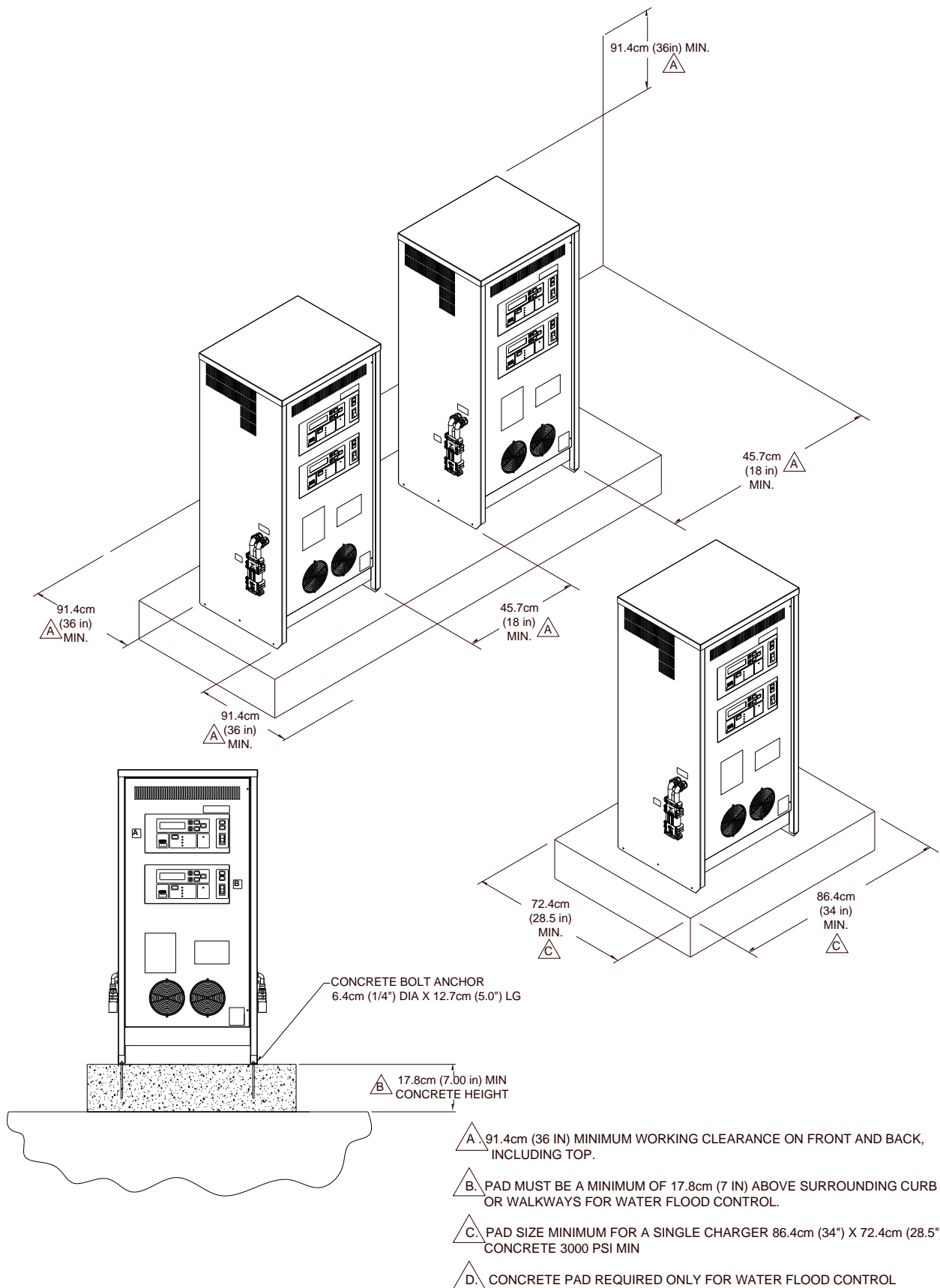
Figure 4- 1 DVS100 Installation
