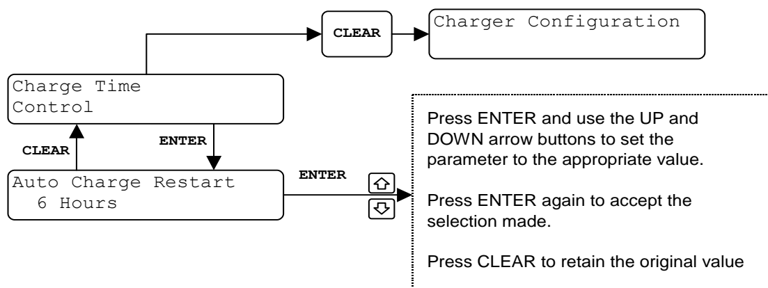
Figure 5- 26 Charger Time Control Menu
