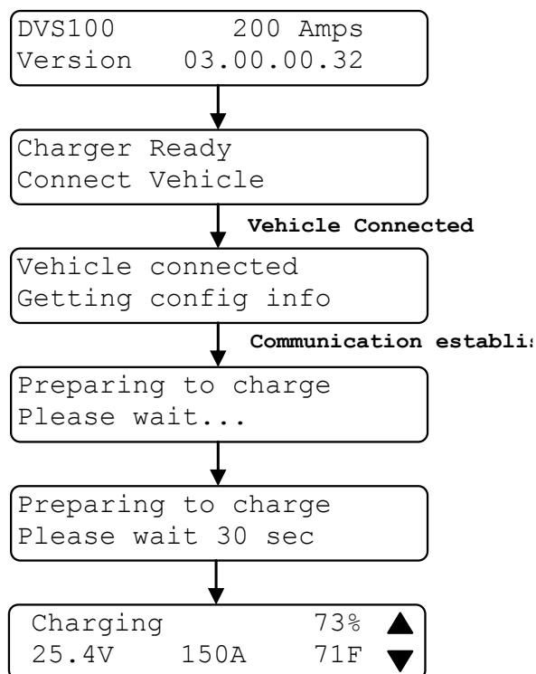
Figure 5- 3 Connecting Status Screens
