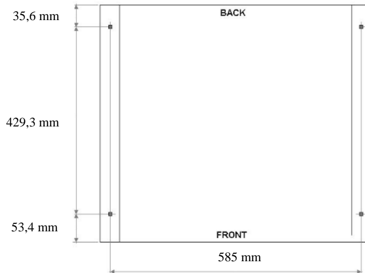
Figure 4- 2 Bolt Pattern for DVS100 Installation
