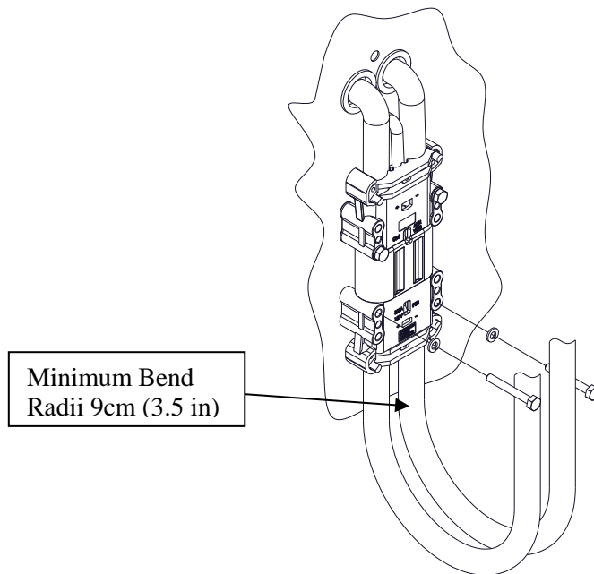
Figure 6- 1 DC Output Cable Installation
