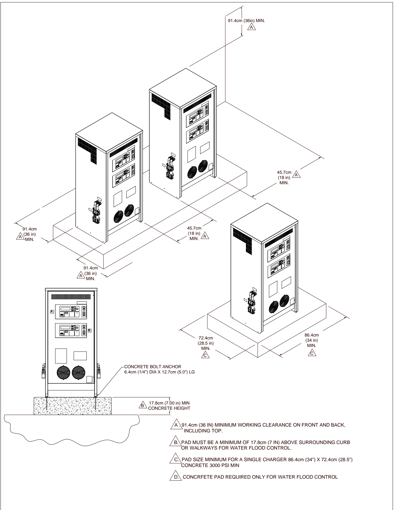
Figure 4- 1 DVS100 Installation
