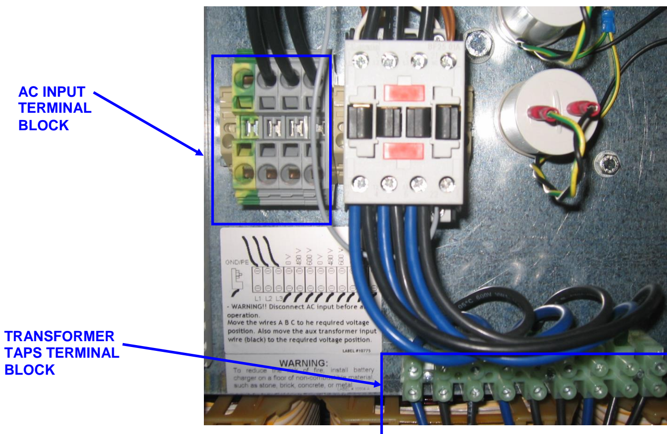
Figure 4- 3 Location of Transformer Taps Terminal Block
