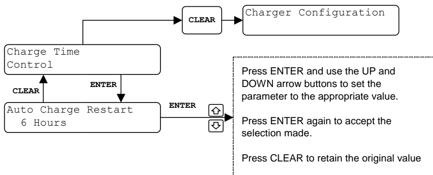
Figure 5- 26 Charger Time Control Menu
