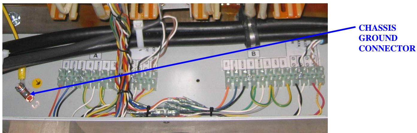
Figure 4- 5 Location of Chassis Ground Connector
