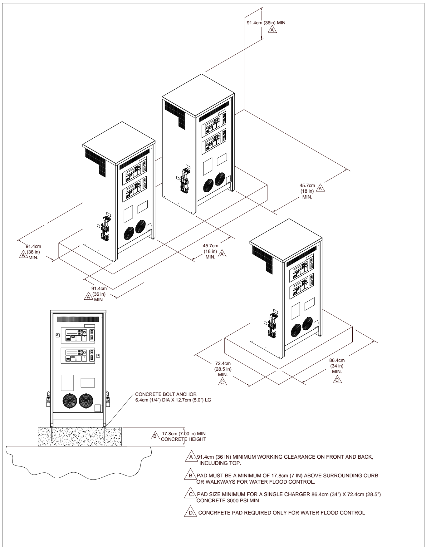
Figure 4- 1 DVS100 Installation
