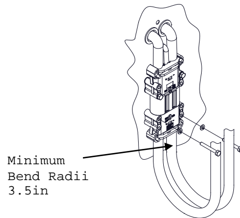
Figure 4-6 DC Output Cable Installation
